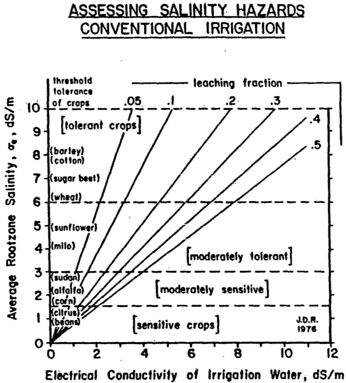
Figure 1 : Relations between average rootzone salinity (saturation extract basis), electrical conductivity of irrigation water, and leaching fraction to use for conditions of conventional irrigation management
