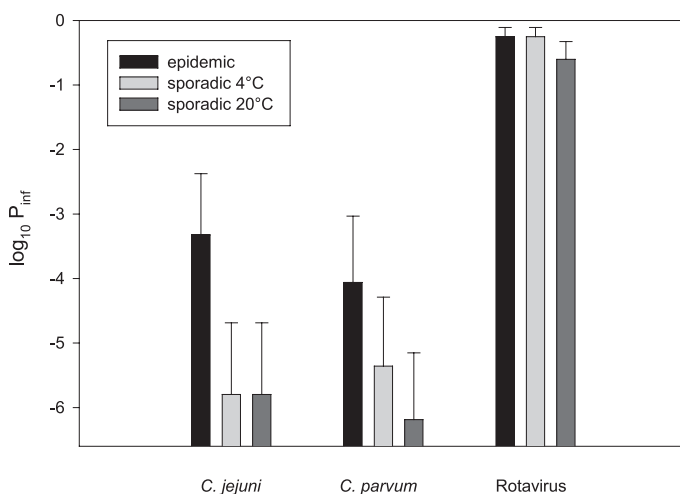
Figure 3.2 Mean probability of infection (5–95%) by Campylobacter jejuni , Cryptosporidium parvum and rotavirus following unintentional ingestion of 1 ml unstored urine for epidemic and sporadic scenarios and 4 °C or 20 °C during collection (Höglund, Ashbolt & Stenström, 2002)
