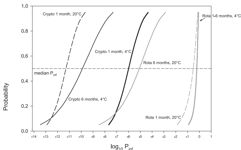
Figure 3.3 Probability of infection (5–95%) by Cryptosporidium parvum and rotavirus following ingestion of 1 ml stored urine (one or six months, 4 °C or 20 °C). C. parvum stored for six months at 20 °C yielded a risk that was <10^{-15} , as did Campylobacter after one month at both temperatures; this information has not been included in the figure (Höglund, Ashbolt & Stenström, 2000).
